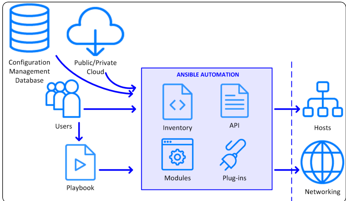
Ansible Architecture
