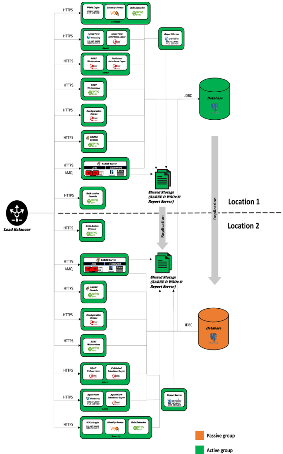
Simple CMP Deployment for High Availability
